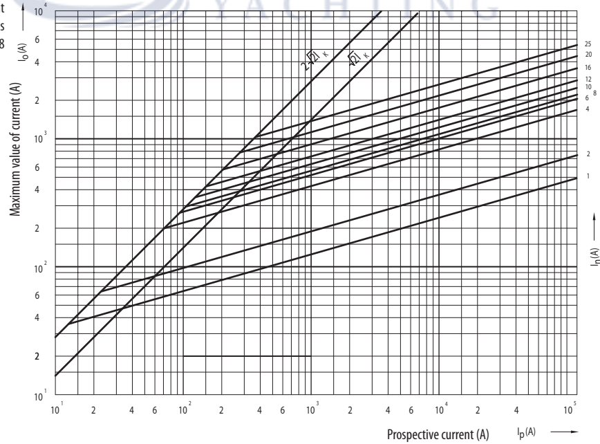
Cut-off current characteristics CH8
